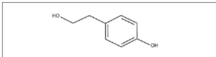
Figure 4—Tyrosol.
