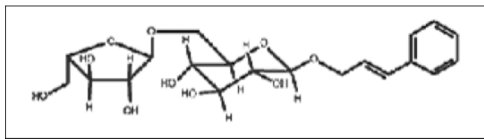
Figure 5—Rosarin.
